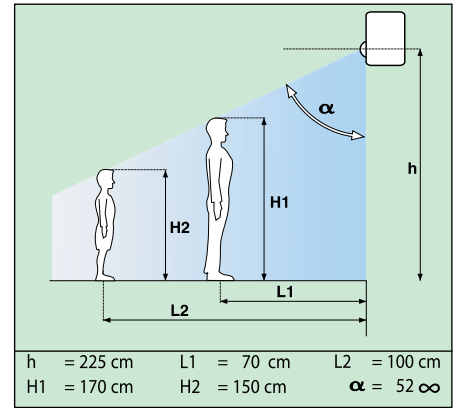
Activation range of PIR detector.
